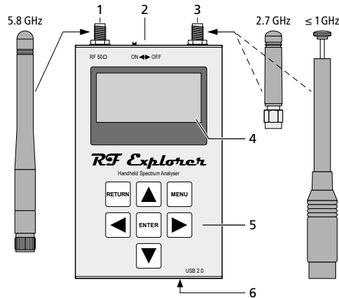
Fig. 1 Connections and operating elements
