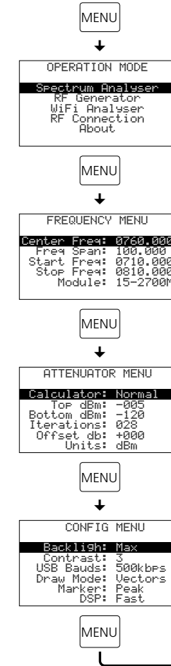
Fig. 4 Menu structure
