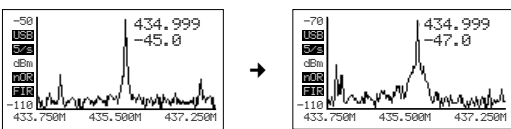
Fig. 12 Upper dBm value reduced by 20 dB
